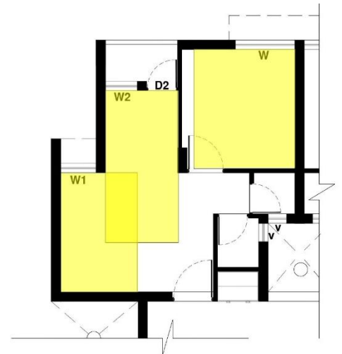
Figure 6: Daylight compliant area (yellow rendered)
